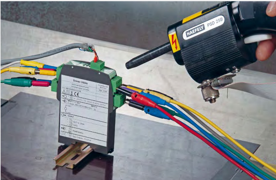
Test of immunity to static discharges on a SINEAX V604s
