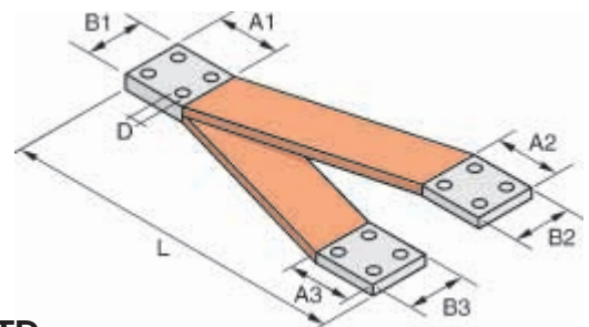
Type TD
