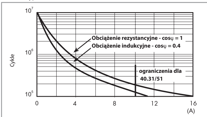
F 40.5 - Electrical life (AC) v contact current Typ 40.11 (strona 5)
