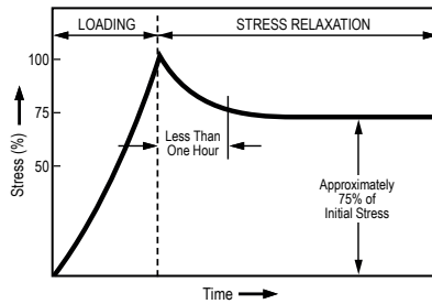
Graph 3-15. Stress Relaxation
