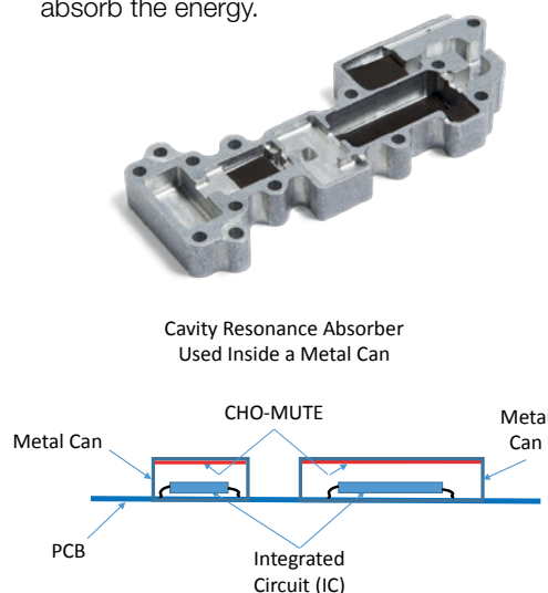
Figure 8-1 Cavity Resonance Absorber Used Inside a Metal Can
