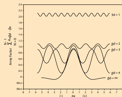
Figure 1-12. Array Factor vs. Spacing
