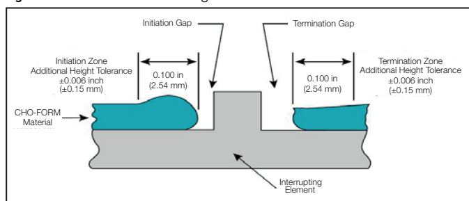
Figure 7-3 Side View Gasket height tolerances
