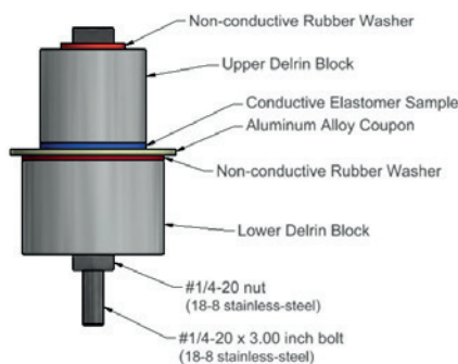
Figure 2-1: Test Fixture
