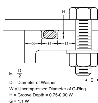
Figure 1-1. Machined Flange with Gasket Groove
