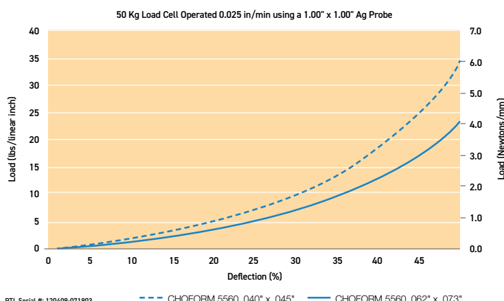
Graph 7-1 Deflection vs. Applied Load
