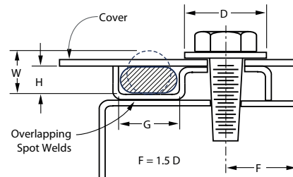
Figure 1-2. Shaped Sheet Metal Container
