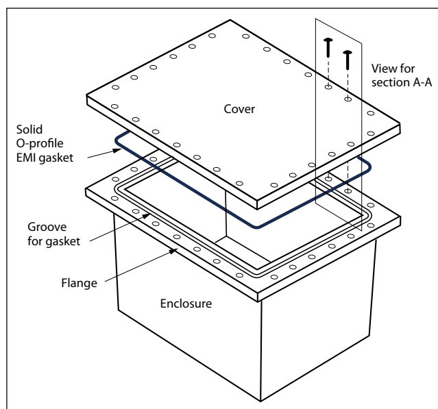
Figure 1-17. Exploded View of Electronic Enclosure
