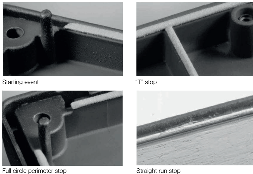
Figure 7-1 Characteristic appearance of start/stop events
