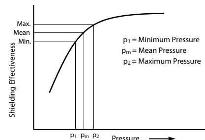
Figure 1-15. Typical Gasket Performance Curve
