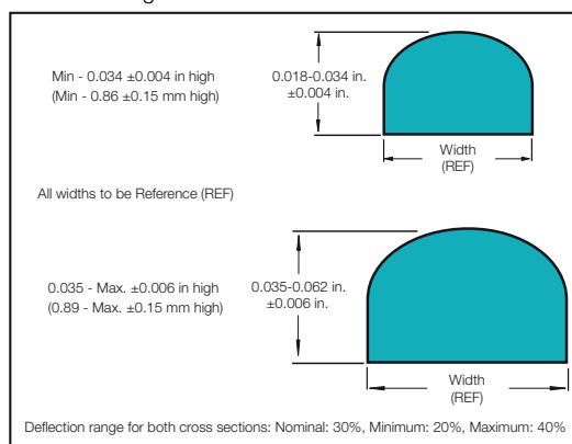
Figure 7-4 Suggested cross sections with height-to-width ratio of 0.85
