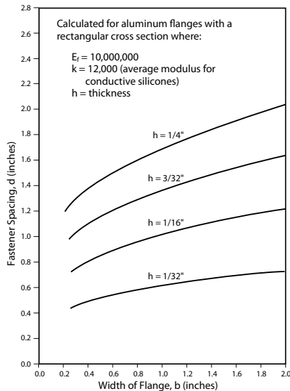
Figure 1-13. Fastener Spacing
