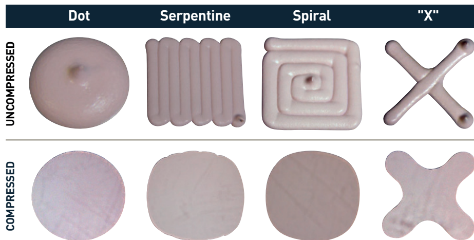
Figure 5: Dispensing Patterns. A simple dot like the first pattern provides adequate coverage, shortest cycle time and least chance of introducing air into the TIM. The more complex the profile, the greater the probability for introducing air (e.g., serpentine and spiral).
