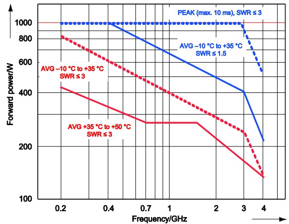
Power-handling capacity
