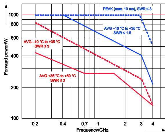
Power-handling capacity
