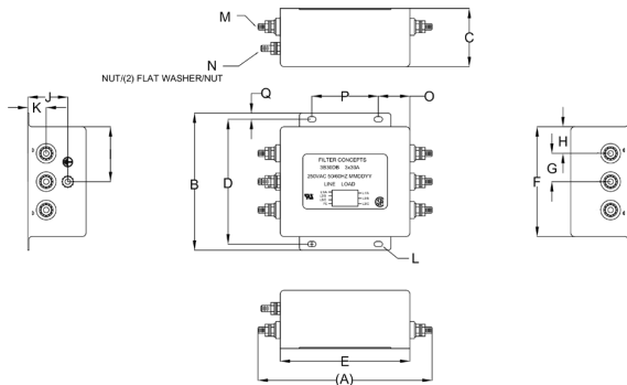
STUDS (30 AMPS)
