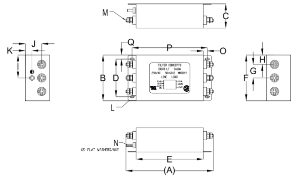
STUDS (60 AMPS)
