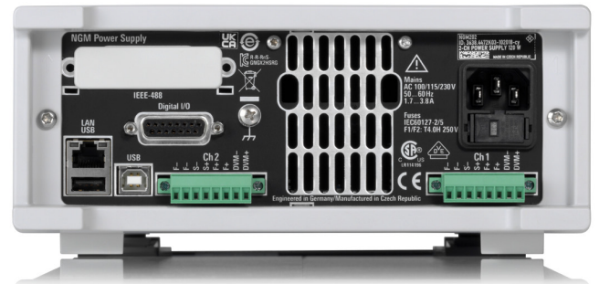
R&S®NGM202, rear view
