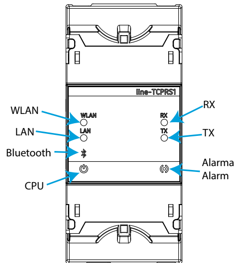
Figure 35: LEDs: line-TCPRS1.
