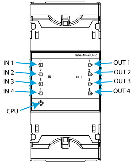
Figure 10: LEDs: line-M-4IO-R.
