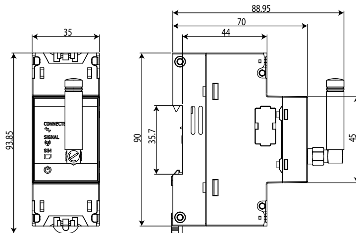
Figure 51: line-M-4G dimensions.
