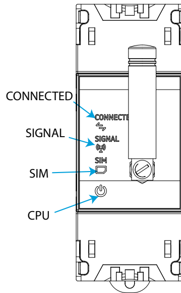
Figure 50: LEDs: line-M-4G.
