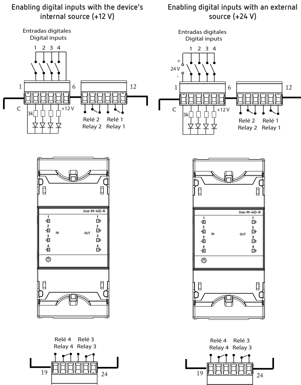
Figure 9: Line-M-4IO-R connection diagram.
