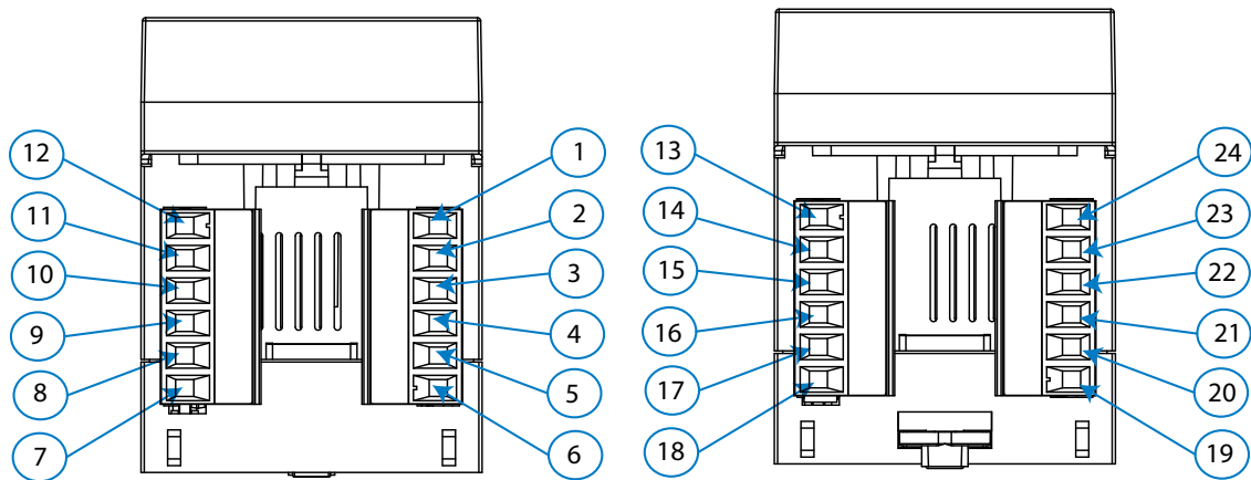
Figure 46: Line-M-8160 terminals: Upper - Lower.
