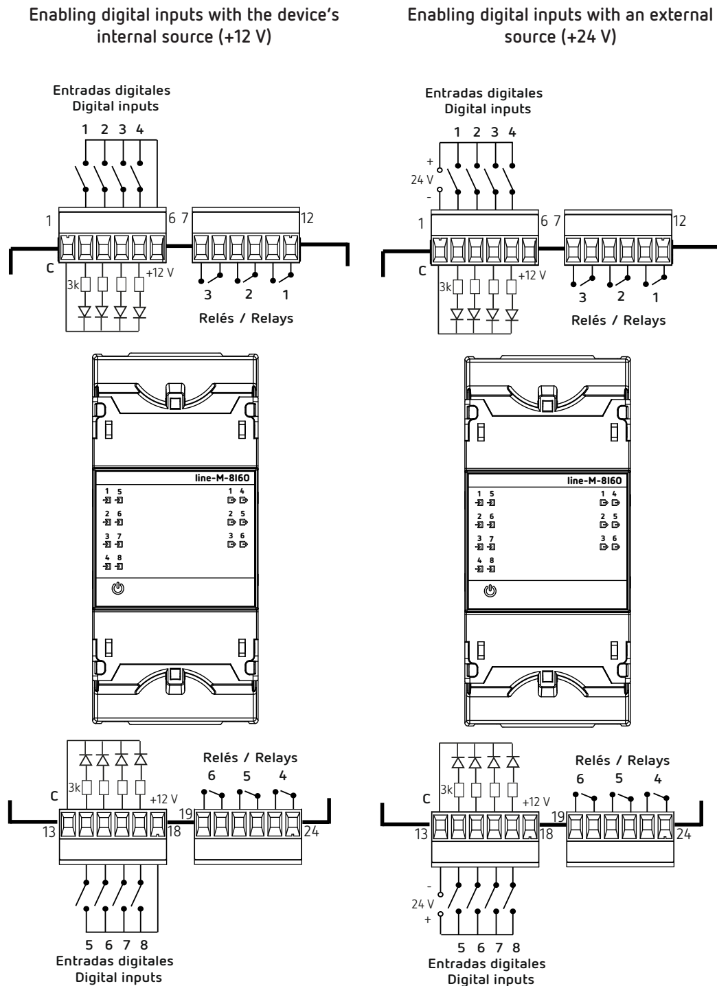
Figure 47: line-M-8160 connection diagram.
