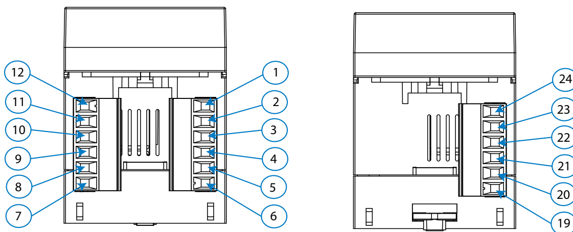
Figure 13: Line-M-4IO-T terminals: Upper - Lower.
