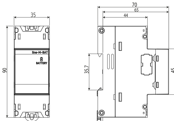
Figure 53: line-M-BAT dimensions.
