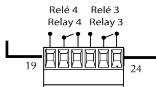
Figure 22: Line-M-410-RV connection diagram.
