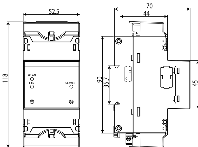
Figure 29: line-EDS-PSxxx dimensions.
