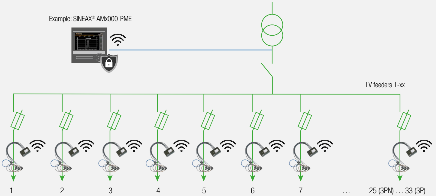
Base station with SINEAX® AM, SINEAX® DM5000, LINAX® PQ or CENTRAX® CU series, incl. integrated Power Monitoring Energy Module (PME) and PME sensors for acquisition of max. 100 currents via radio signal.
