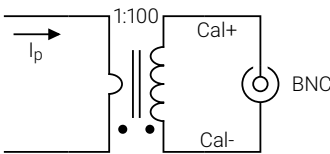
Figure 9: BNC Calibration winding connection
