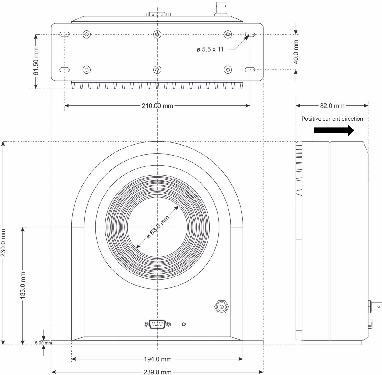
Figure 5: Dimensions of transducer. 0.3 mm Tolerance
