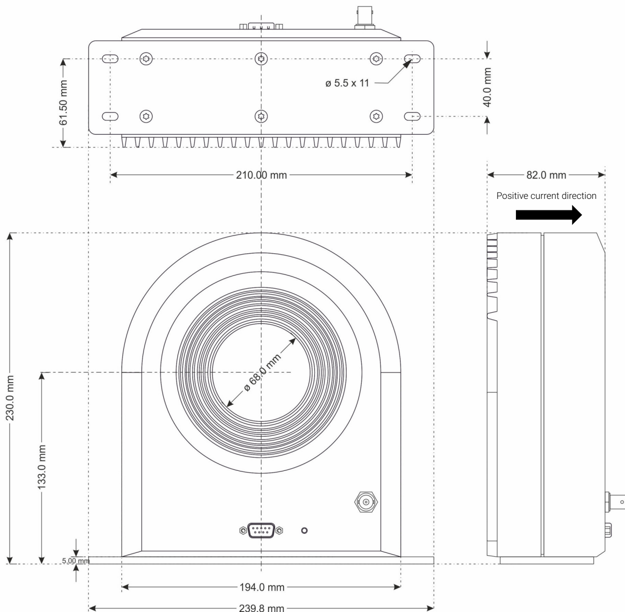
Figure 4: Dimensions of transducer. 0.3 mm Tolerance
