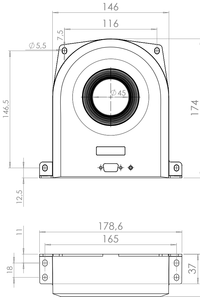
Figure 5: Dimensions of sensor head. Tolerance is 0.3 mm
