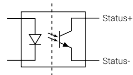
Figure 8: Status signal optocoupler
