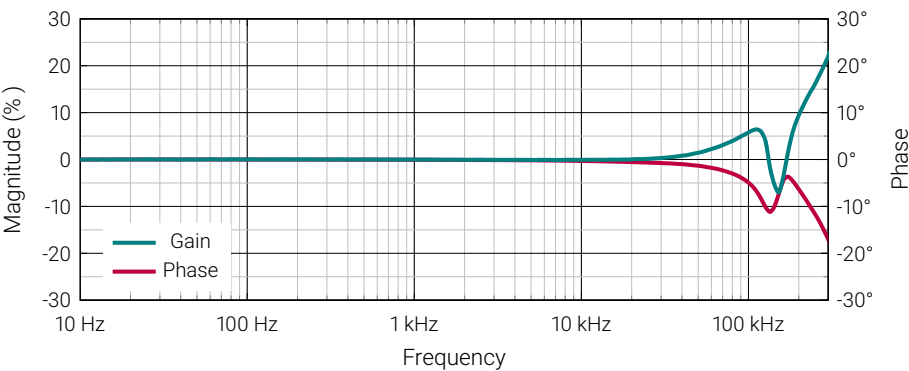
Figure 3: Frequency characteristics
