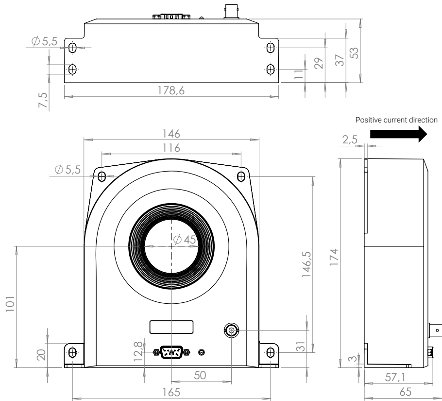
Figure 5: Dimensions of sensor head. Tolerance is 0.3 mm
