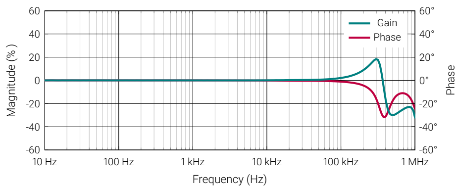
Figure 5: Frequency characteristics
