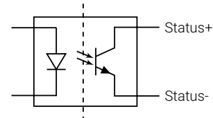
Figure 8: Status signal optocoupler
