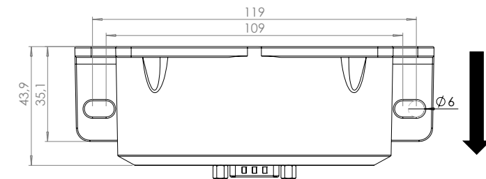
Figure 6: Dimensions of transducer. 0.3 mm Tolerance
