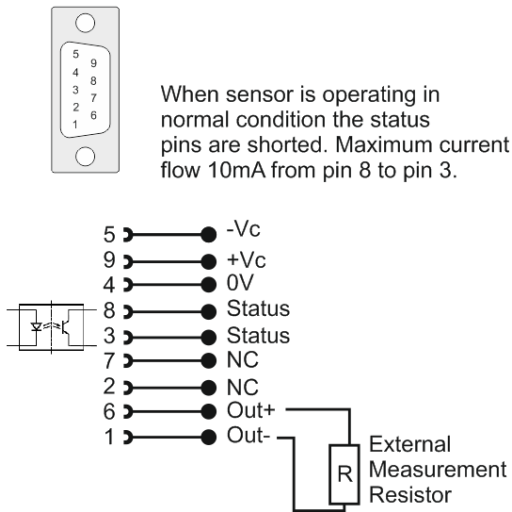
Standard DSUB-9 current output
