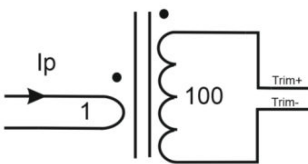
Calibration winding in DSUB-25
