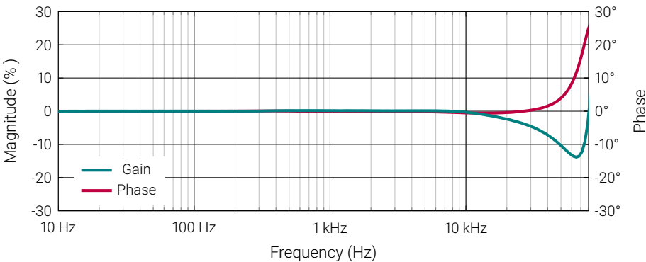
Figure 4: Frequency characteristics
