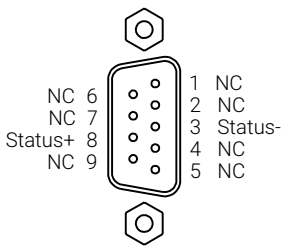
Figure 7: D-sub-9 connection pinout
