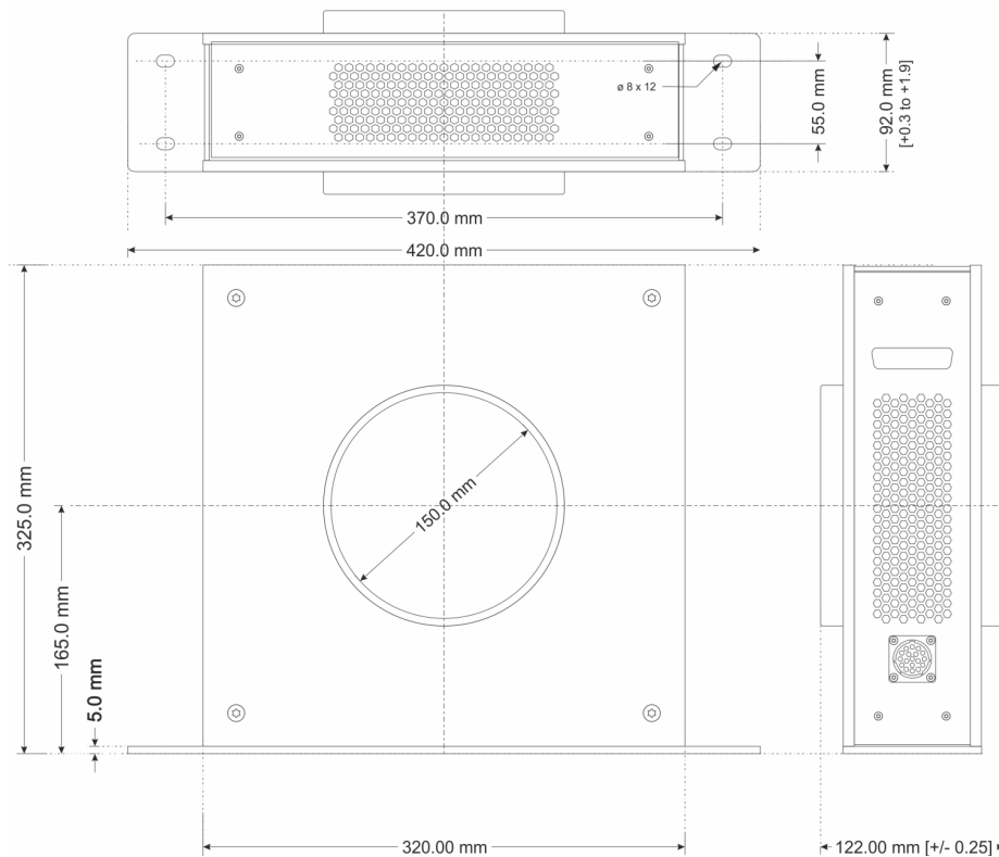
Figure 5: Dimensions of transducer head. 0.3 mm Tolerance
