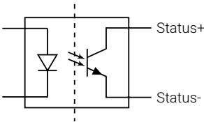
Figure 9: Status signal optocoupler
