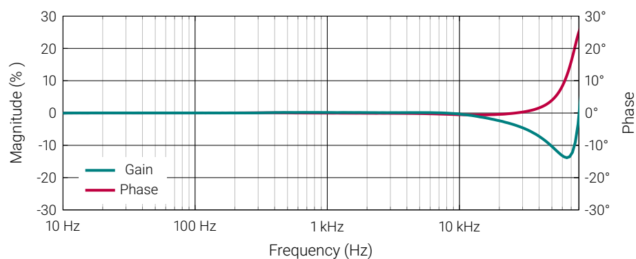
Figure 3: Frequency characteristics
