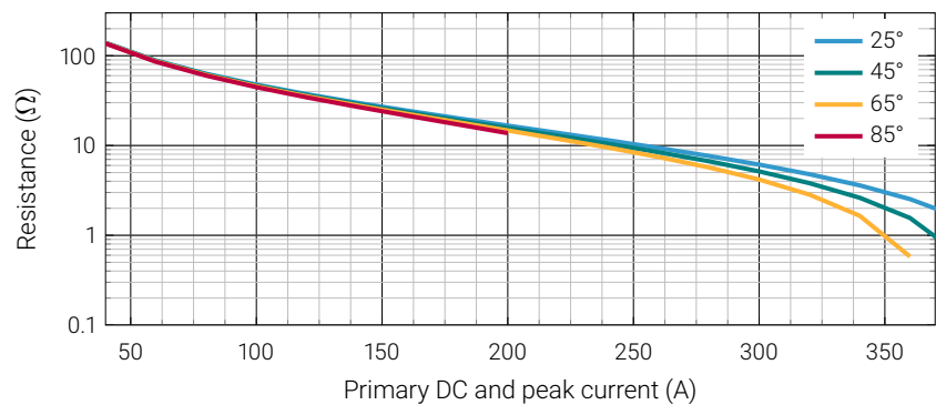
Figure 2: Maximum measurement resistor R_M vs. ambient temperatures
