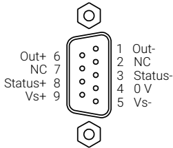
Figure 7: D-sub-9 connection pinout
