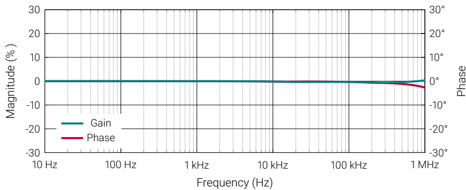
Figure 4: Frequency characteristics
