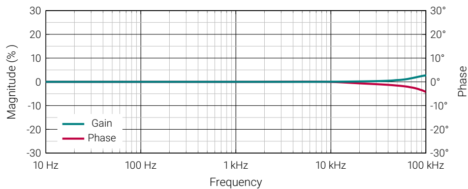
Figure 3: Frequency characteristics
