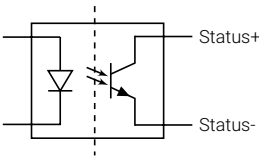
Figure 8: Status signal optocoupler
