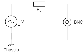
Figure 6: BNC shield and chassis connection
