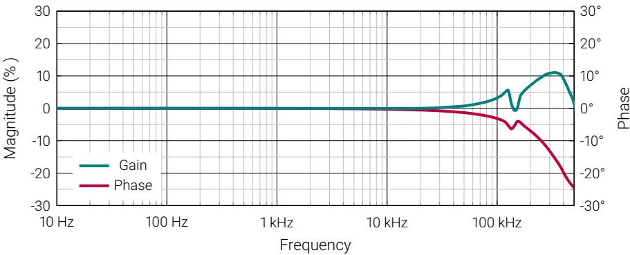
Figure 3: Frequency characteristics
