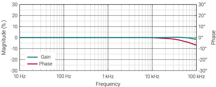
Figure 3: Frequency characteristics
