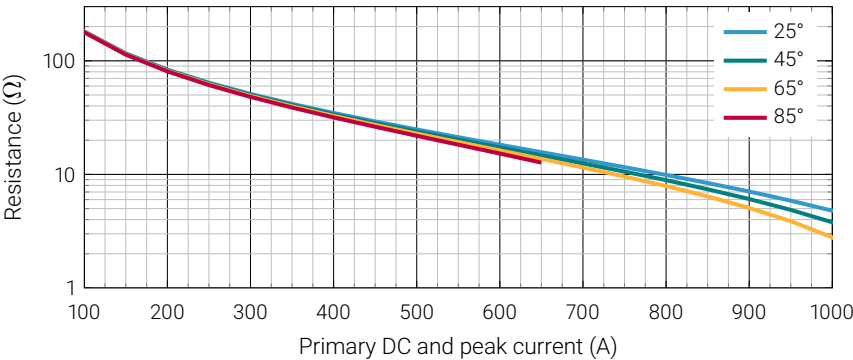
Figure 2: Maximum measurement resistor R_M vs. ambient temperatures
