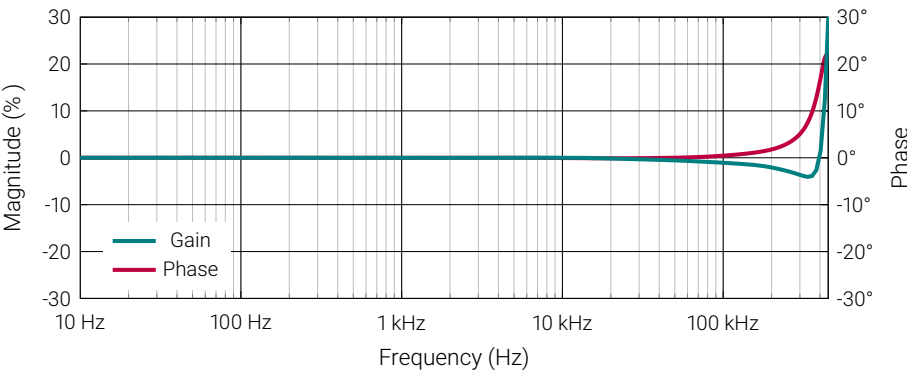
Figure 4: Frequency characteristics
