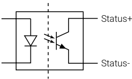
Figure 2: Status signal optocoupler
