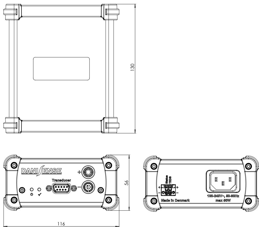
Figure 3: Box dimensions
