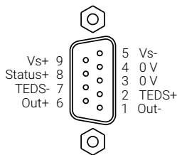
Figure 1: D-sub-9 female connection pinout
