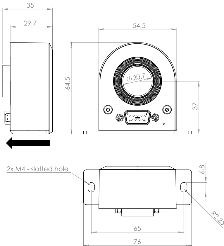
Figure 5: Dimensions of transducer. 0.3 mm Tolerance
