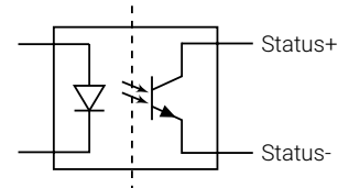
Figure 7: Status signal optocoupler
