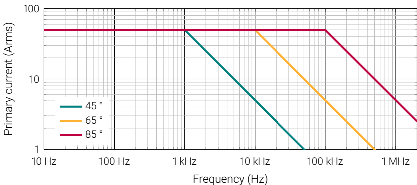
Figure 3: Maximum continuous primary current vs. frequency
