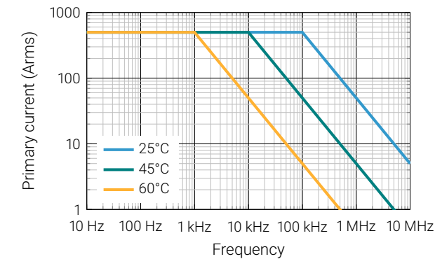
Figure 2: Maximum continuous primary current vs. frequency
