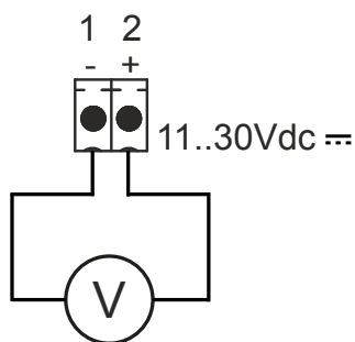
Connection scheme BT7050
