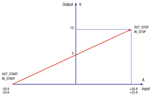
Input / Output Bipolar
