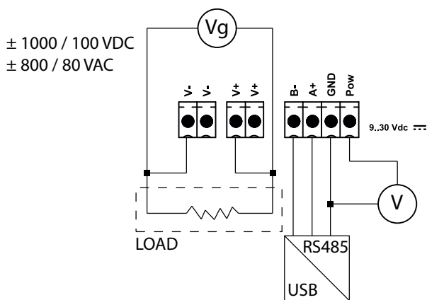
Connection scheme BT7300 / BT7350
