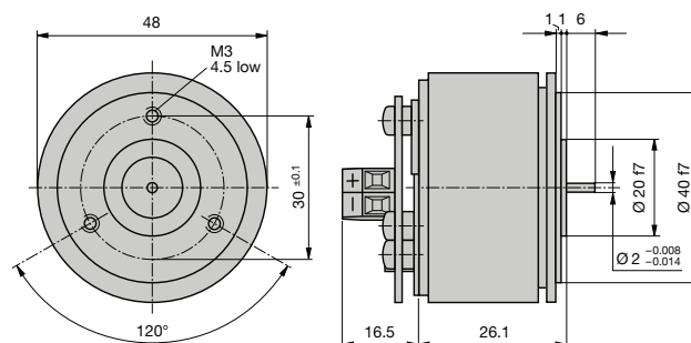
Fig. 1. KINAX 2W2 with standard drive shaft at front only , dia. 2 mm, length 6 mm, screw terminal versions
