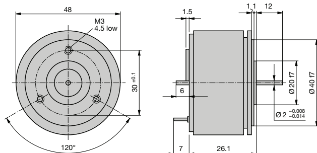
Fig. 2. KINAX 2W2 with special shaft drive at front and at rear. At front: dia. 2 mm, length 12 mm. At rear: dia. 2 mm, length 6 mm.
