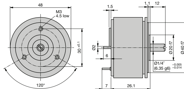
Fig. 6. KINAX 2W2 with special drive shaft at front and at rear. At front dia. 1/4", length 12 mm. At rear dia. 2 mm, length 6 mm.
