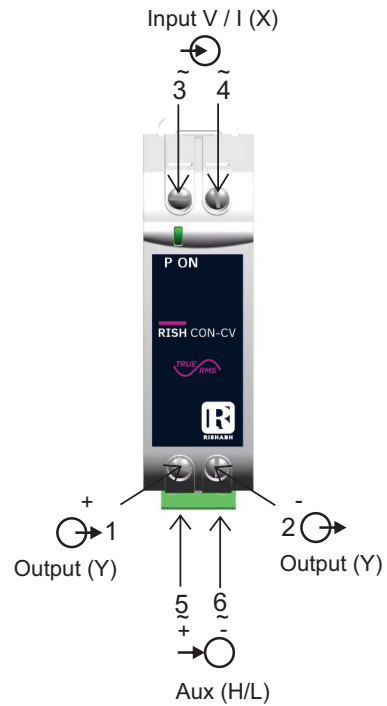
Fig. 3. RISH CON - CV/CA Connection Diagram.
