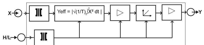
Fig. 2. Block Diagram.
