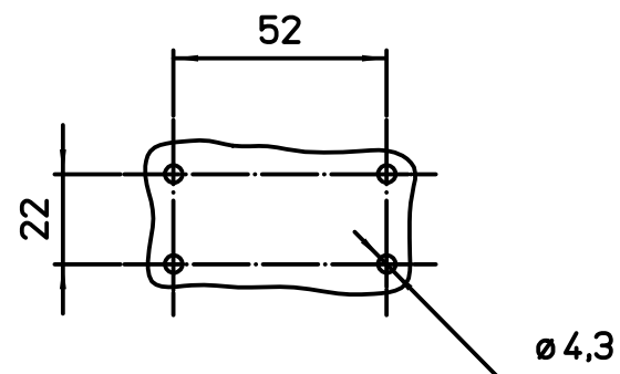
Panel cut-out
