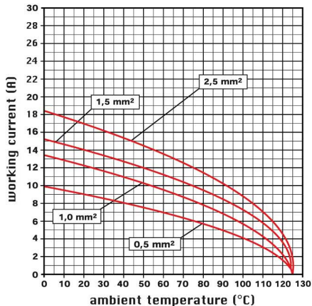
diagram CSH 24 poles
