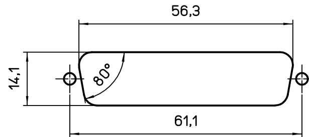
Rear mounting panel cut-out
