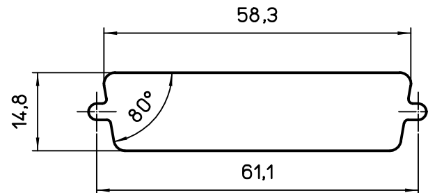
Front mounting panel cut-out
