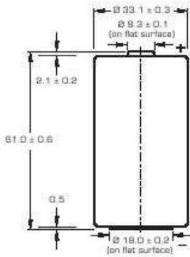
Finished version with protruding positive end cap
