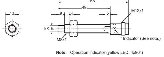
E2A-S08LN04-M1-□□
