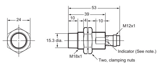
E2A-S18KN16-M1-□
