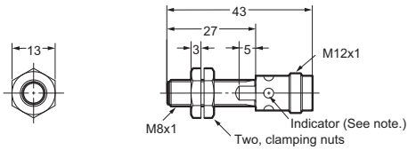
E2A-S08KS02-M1-□□
