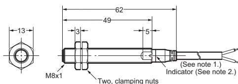
E2A-S08LS02-WP-□□
