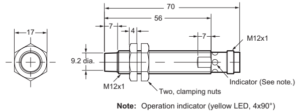
E2A-S12LN08-M1-□
