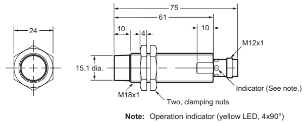
E2A-S18LN16-M1-□
