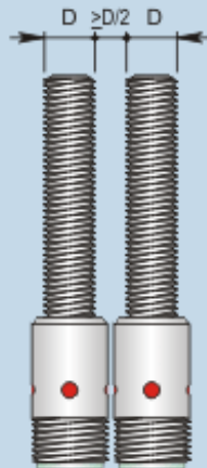
Side by side mounting
