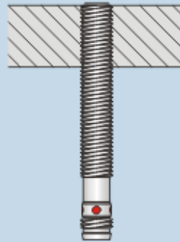
Flush mounting
