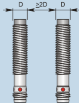
Side by side mounting
