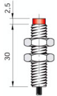
Dimension in mm
