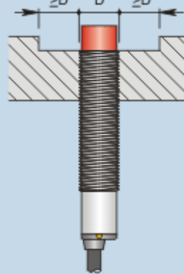
Non flush mounting
