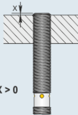
Flush mounting
