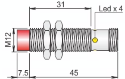
Dimension in mm
