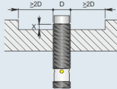
Non flush mounting
