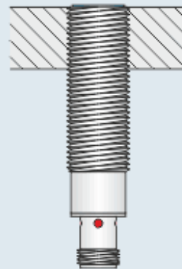
Flush mounting
