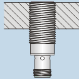
Flush mounting
