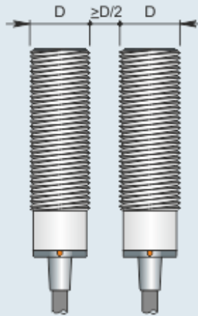
Side by side mounting
